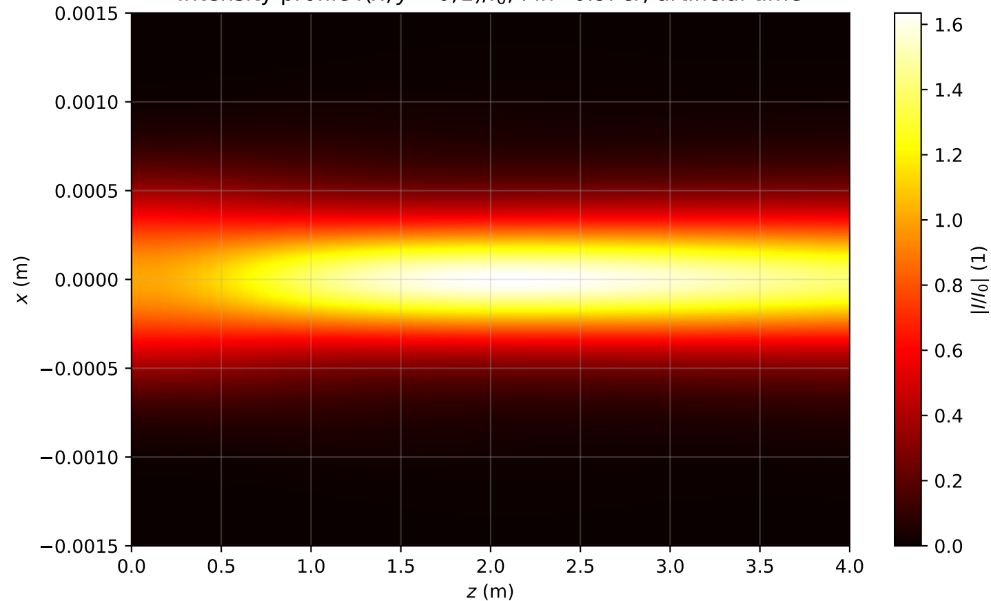
Intensity profile I(x, y = 0, z)/I_0 , P_{in}=0.9P_{cr} , artificial time
